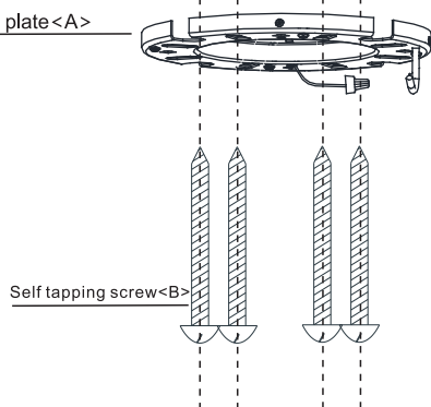
Mounting plate<A>
